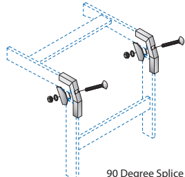
90 Degree Splice Kit
