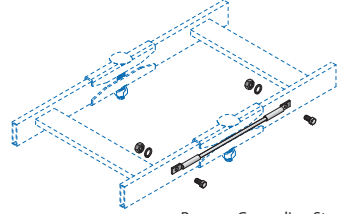
Runway Grounding Strap
