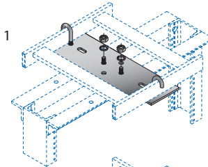
Elevation Kit
