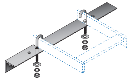
Wall Angle Support Kit
